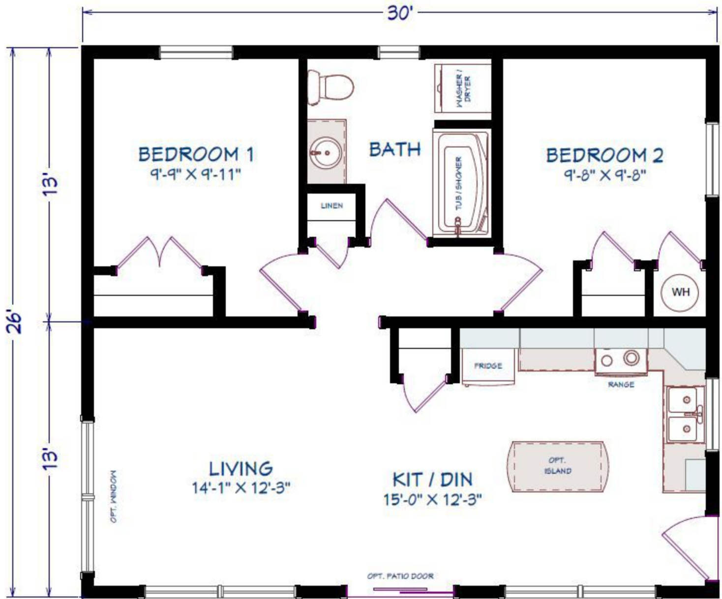
2 BEDROOMS, 1 BATHROOM 780 SQ FT
